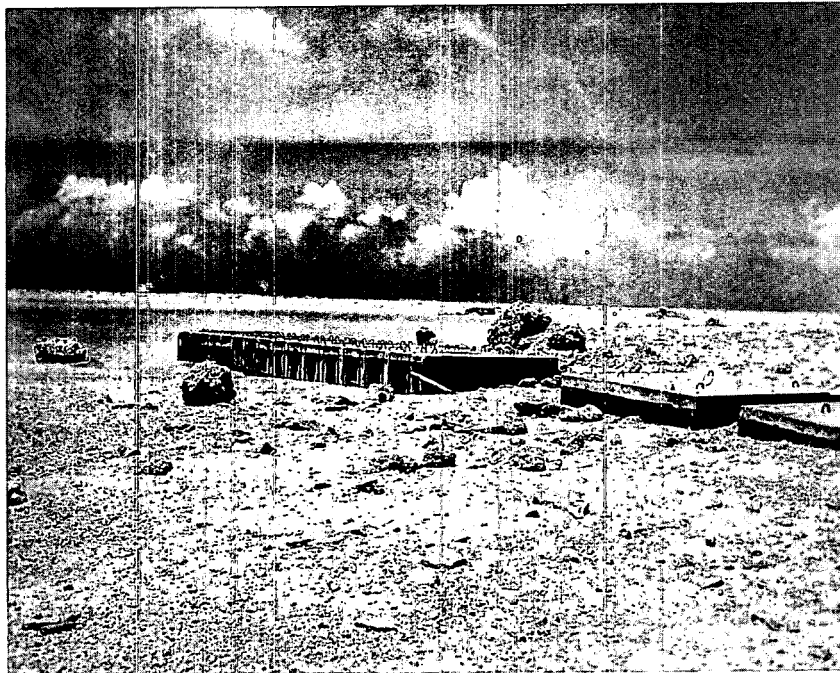
Fig. 8—Posttest view of one-way slabs at station 360.01, range 1830 ft, looking at GZ side of slabs.
